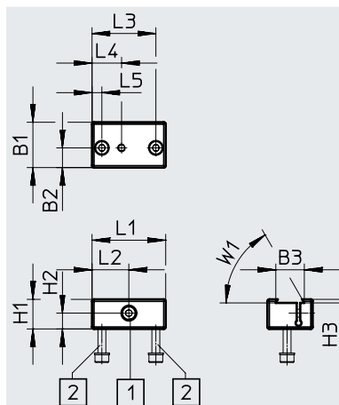
[1] Schraube M4x12
